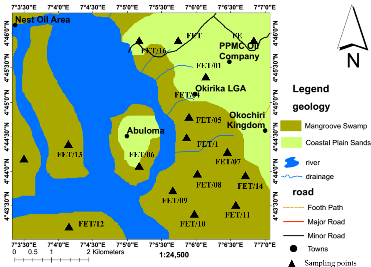
Fig. 2: Geology map of the study.
