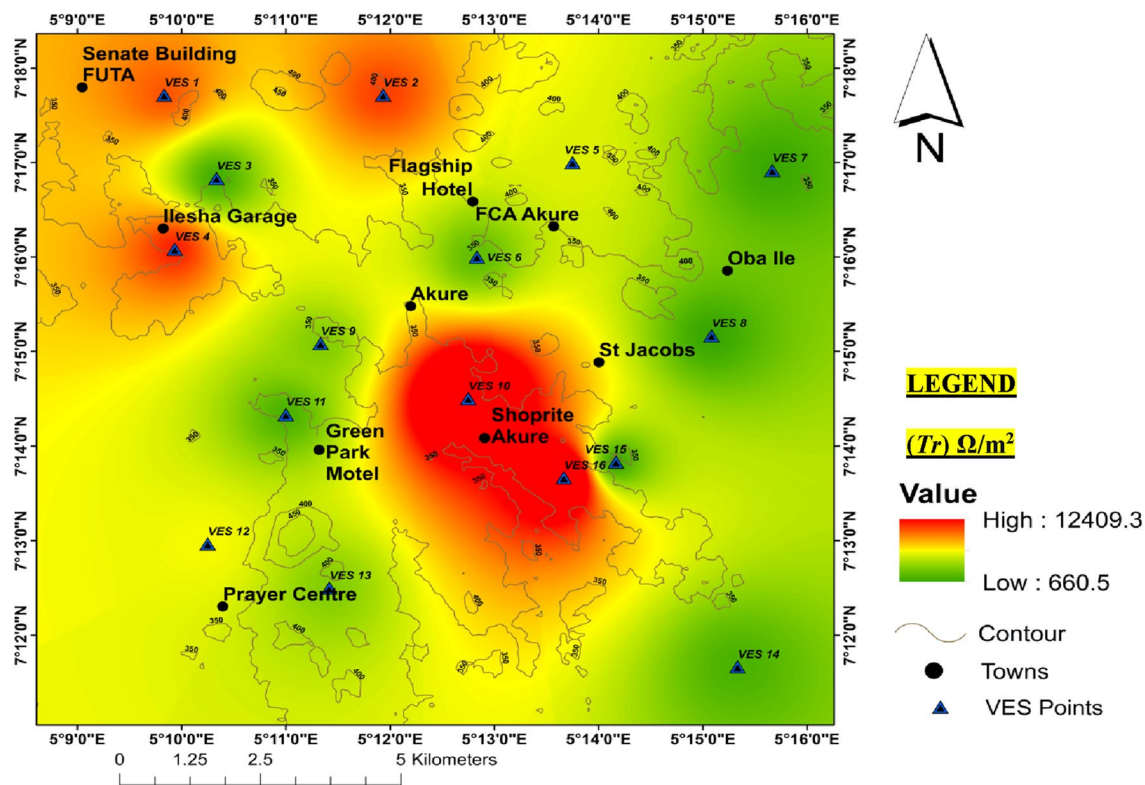
Fig. 3 Spatial distribution map of transverse unit resistance
