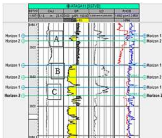
Fig. 9: Well Panel showing Reservoir A, B and C
