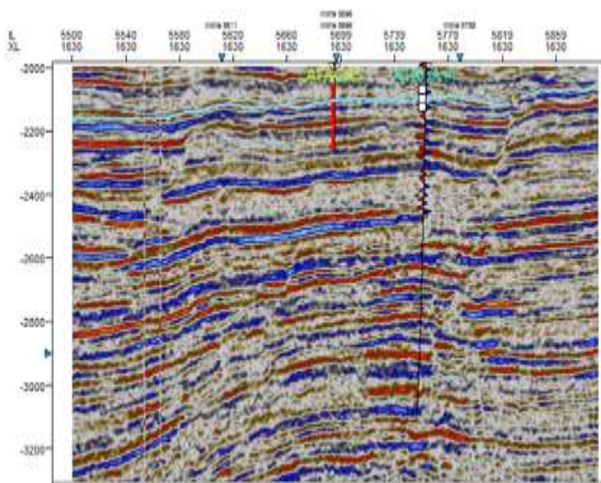
Fig. 3: Seismic section showing synthetic seismogram tying with well ATA 11
