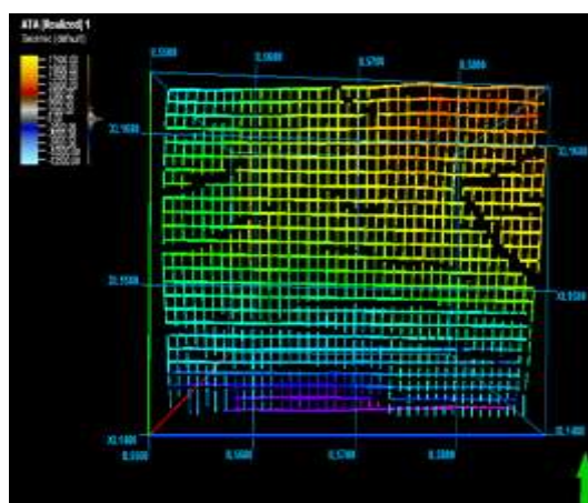
Fig. 6: 3-D window showing the mapped horizons for Reservoir B
