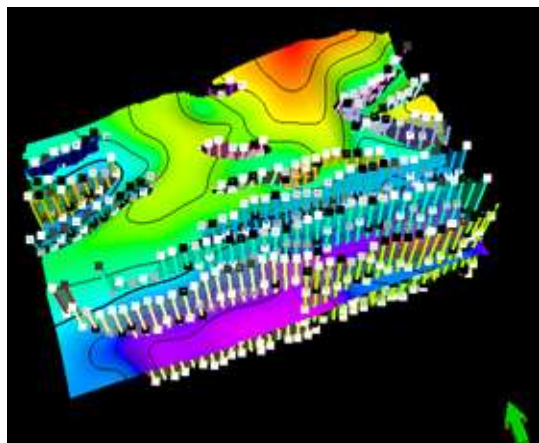
Fig. 5: 3-D window showing the fault interpretation on the structural map
