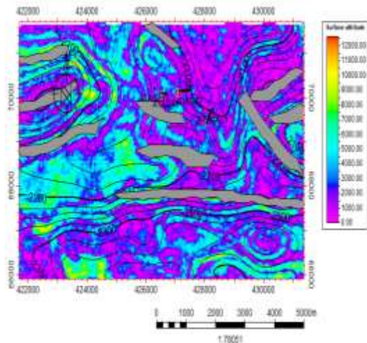
Fig. 8: Amplitude attribute map of Reservoir B
