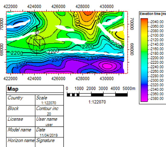
Fig. 7: Time Structural map generated from the mapped horizon of Reservoir B
