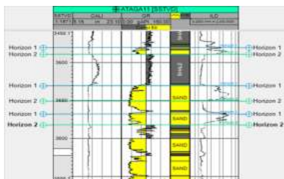
Fig. 11: Well panel showing the Lithofacies and the payzones in ATA1
