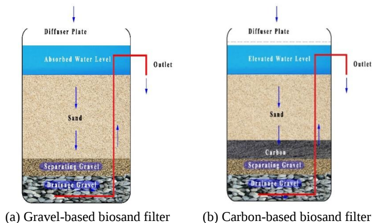
Figure 2: Biosand filter
