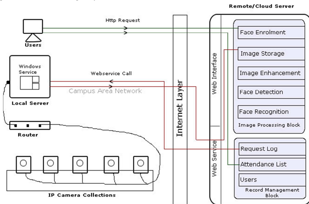
Figure 4. FACECUBE architecture.
