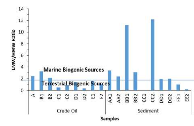
Fig. 4. Plot of LMW/HMW n-alkanes in the crude oil against sediment samples
