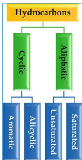
Fig. 1. Hydrocarbons classification (Muharrem and Olcay, 2019)
