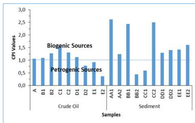
Fig. 5. CPI values of aliphatic hydrocarbons in crude oil and sediment samples
