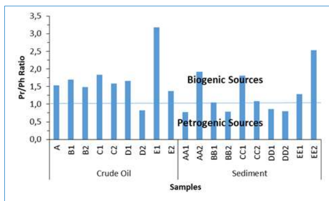
Fig. 6. Pr/Ph ratio of aliphatic hydrocarbons in the crude oil and sediment samples
